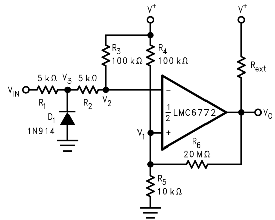
FIGURE 7. Zero Crossing Detector
