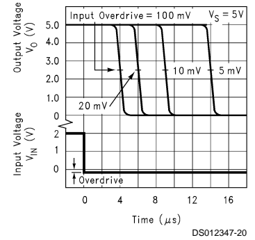
Response Time for Overdrive ( t_{PHL} )
