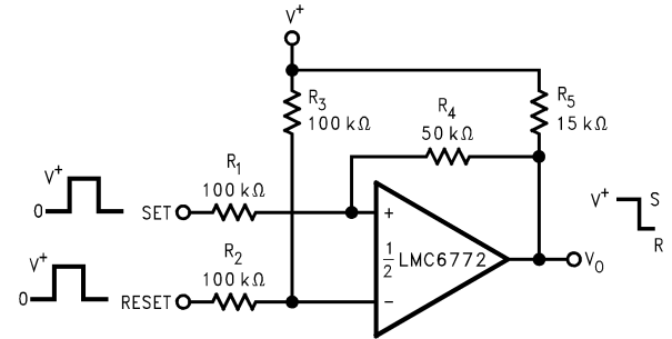
FIGURE 6. Bi-Stable Multivibrator
